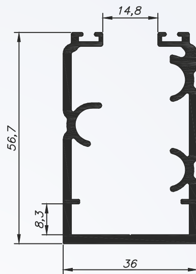
JP-026 6,800 Kg/BARRA 6m
