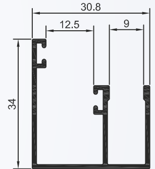
BX-214 2,190 Kg/BARRA 6m
