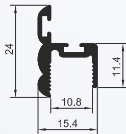
BX-209 1,500 Kg/BARRA 6m
