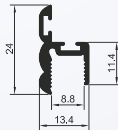
BX-261 1,390 Kg/BARRA 6m
