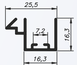
DS-1391 1,310 Kg/BARRA 6m
